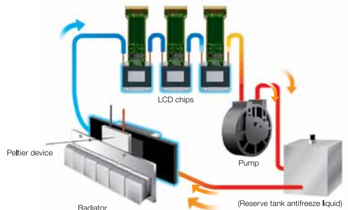
▲ Hybrid cooling system
