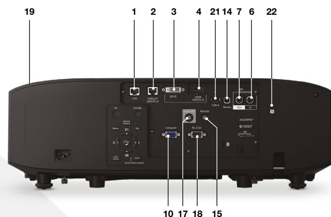
Model shown is the EB-PU2010B
